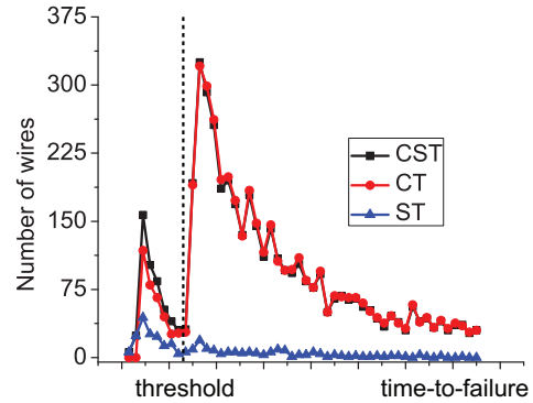
Fig. 13. Wire distribution in according to failure time. The vertical line divides the critical region from the non-critical region.
