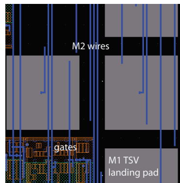
Fig. 1. Typical layout of 3D IC, where TSV landing pads in M1, gates, and M2 are shown. M2 wires going over or running nearby are under the risk of EM-related failure due to TSV-induced stress.
