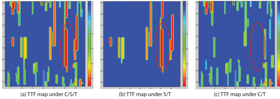
Fig. 12. Zoom in image of the layout shown in Figure 11. (a) Map of critical wires when considering current, stress, and temperature. (b) Map of critical wires when considering stress, and temperature. (c) Map of critical wires when considering current, and temperature. Highlighted regions shows a failure hot-spot that occurs due to TSV induced stress.
