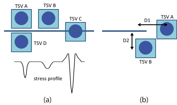
Fig. 8. Stress profile on a wire due to multiple TSVs. (a) When the TSVs are located in regions far away from the end points of a wire. (b) The end point may experience positive or negative stress gradient based on how far it is from TSV A ( D1 ) or from TSV B ( D2 ).
