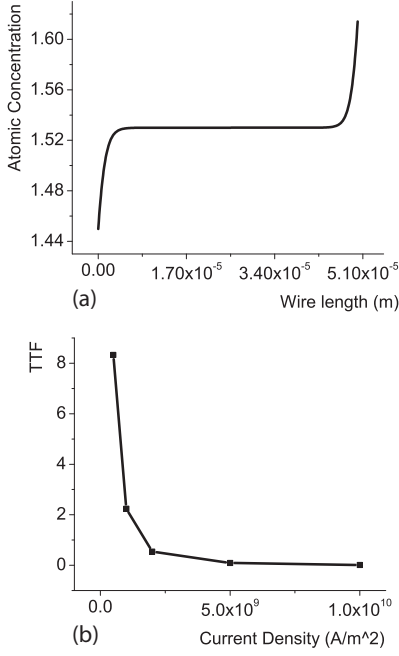
Fig. 2. (a) Change in concentration along a wire due to current. (b) Impact of current density on failure time of a metal wire.
