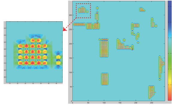
Fig. 10. Variation of hydrostatic stress for vertical wires on a given die.
