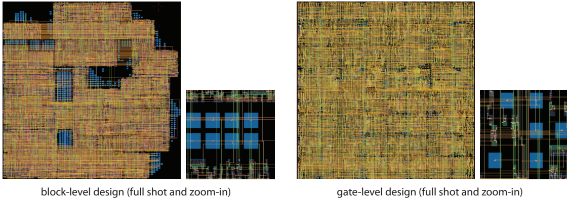
Fig. 14. GDSII layout shots of our block-level vs gate-level designs.
