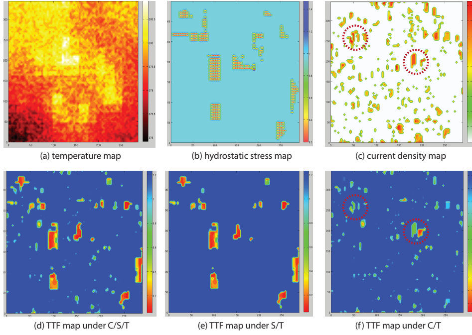
Fig. 11. (a) Temperature map. (b) Map of variation of hydrostatic stress for vertical wires. (c) Map of current density. (d) Map of critical wires when considering current, stress, and temperature. (e) Map of critical wires when considering stress, and temperature. (f) Map of critical wires when considering current, and temperature. Circled regions in (c) and (f) show that high current density region correspond to critical locations.
