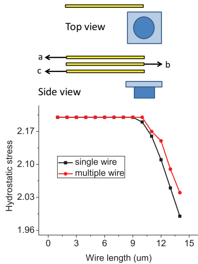
Fig. 7. Impact of nearby metallization. We plot the stress profile of wire 'b' for two cases: 1) when wires 'a' and 'c' are present during simulation (multiple wire), and 2) when wires 'a' and 'c' are absent during simulation.
