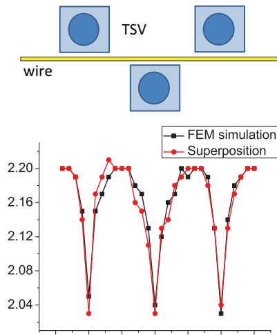
Fig. 6. Comparison between superposition-based stress calculation and FEM-based stress calculation.
