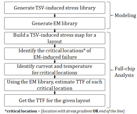
Fig. 9. Generating libraries and estimate the EM time-to-failure for a full-chip layout based on the libraries.
