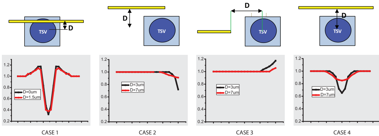
Fig. 5. 4 different cases of a horizontal wire location with respect to a TSV. The top row shows the top view of these cases, where we show a thin horizontal wire, circular TSV and its landing pad. The bottom row shows the stress profile on the wire. It also shows the impact of TSV stress based on the distance D between the wire and TSV.
