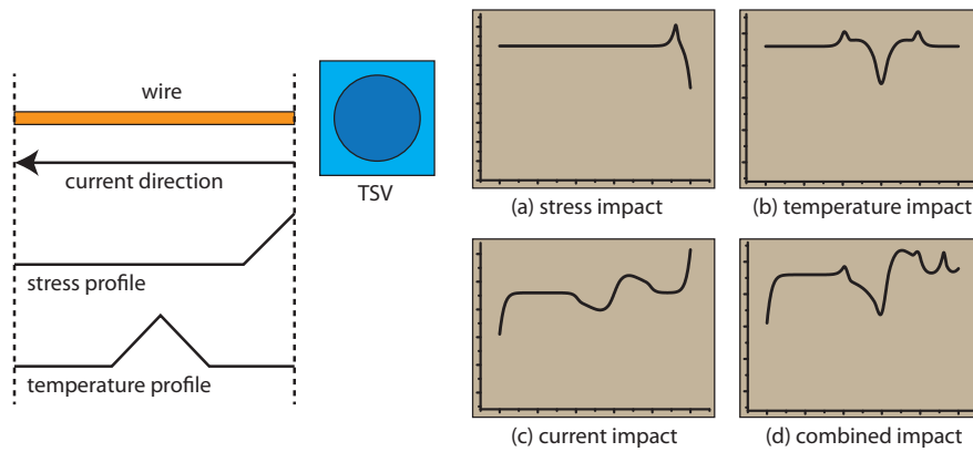
Fig. 4. A single wire subject to current, stress profile and temperature profile. (a) Change in atomic concentration due to stress gradient. (b) Change in atomic concentration due to temperature gradient. (c) Change in atomic concentration due to current. (d) Change in atomic concentration due to combined effect of all three forces.
