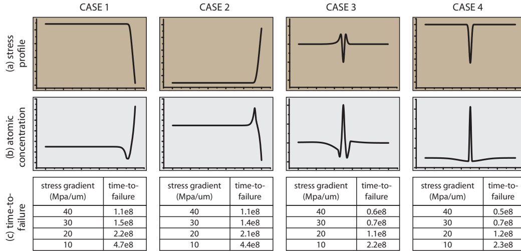
Fig. 3. (a) Four different stress profiles acting on a wire. (b) Change in atomic concentration due to stress gradients. (c) Impact on time-to-failure due to increasing stress gradient.
