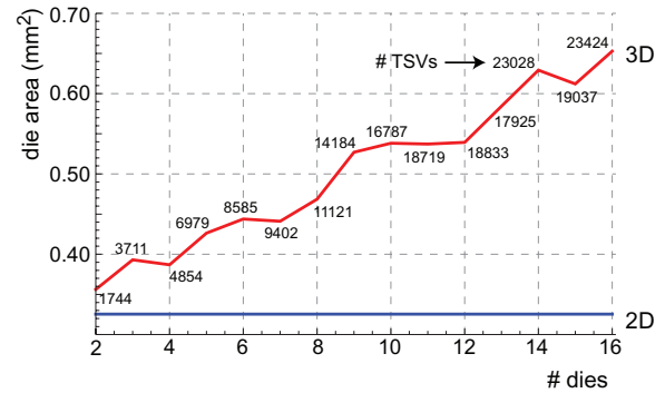
Figure 11: Die area and # TSVs of des_perf in 3D design
