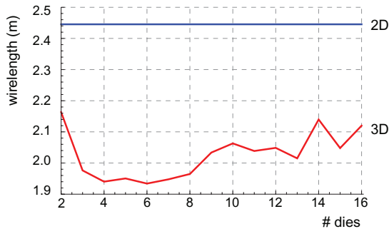
Figure 10: Wirelength vs # dies of des_perf in 3D design
