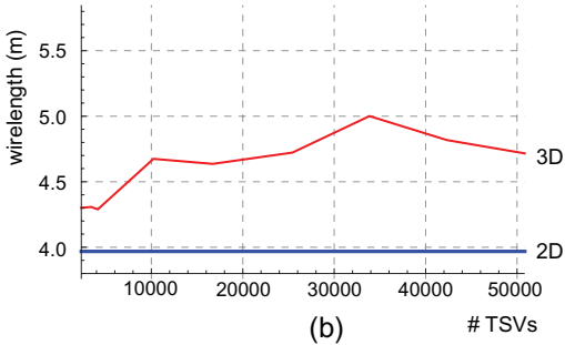
Figure 9: Wirelength vs # TSVs of (a) des_perf, and (b) b19 for 2D and 3D (4 dies) designs
